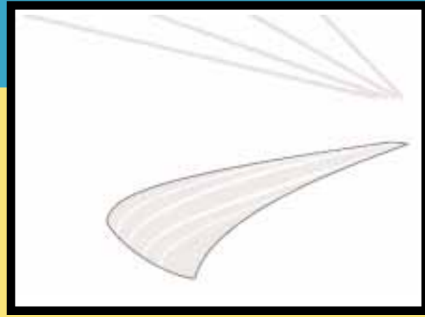
Figure 4. A set of "bad" reflection lines.
