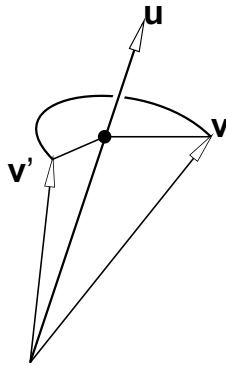
Figure 1: The vector \mathbf{v} is rotated into \mathbf{v}' around axis \mathbf{u} .
