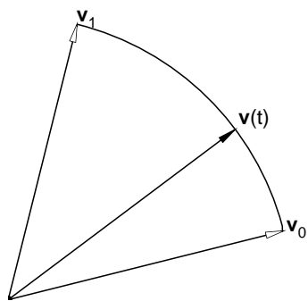
Figure 2: Rotation interpolation in 3D.
